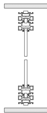
CENTRAL FLIPPING PIVOT System with central pivot
