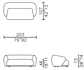
sofa 200
