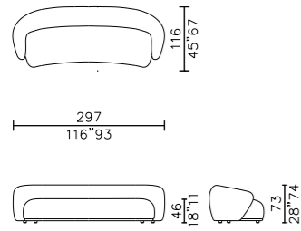
sofa 300 CURVED
