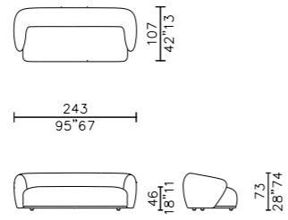
sofa 240
